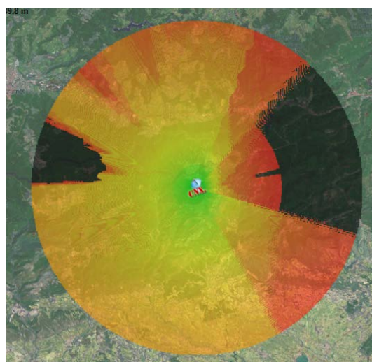
BVLOS telecom signal strength
